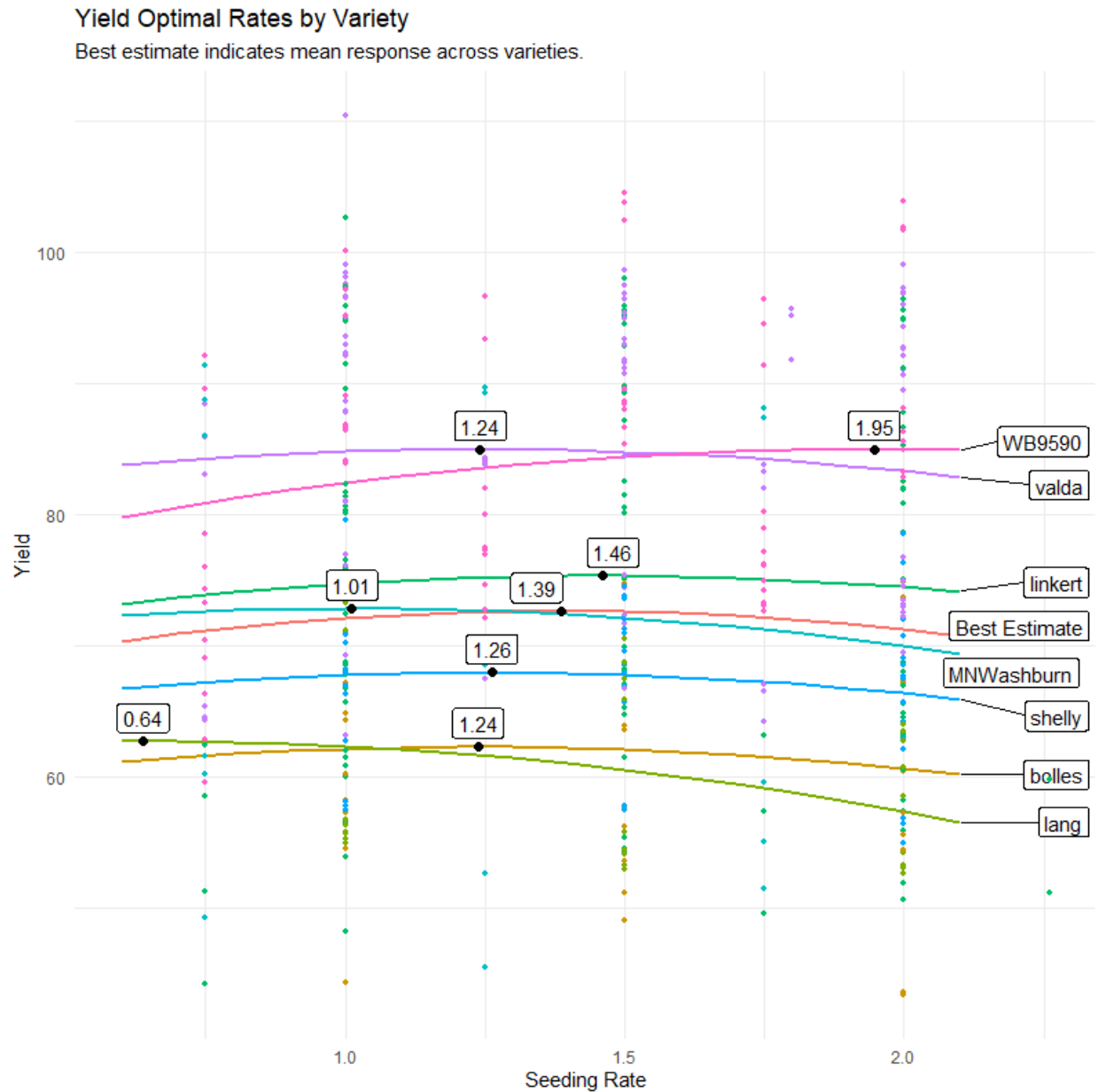
Figure 7. Optimal seeding rate to maximize yield for each variety, using the combined location data from 2016-2020. The number of locations for each variety included in the analysis: Bolles = 4, Linkert = 10, Shelly = 5, Lang-MN = 3, WB9590 = 7, SY Valda = 10, MN-Washburn = 2. Results for varieties with many locations of data will be more reliable than varieties that have only a few locations tested.
